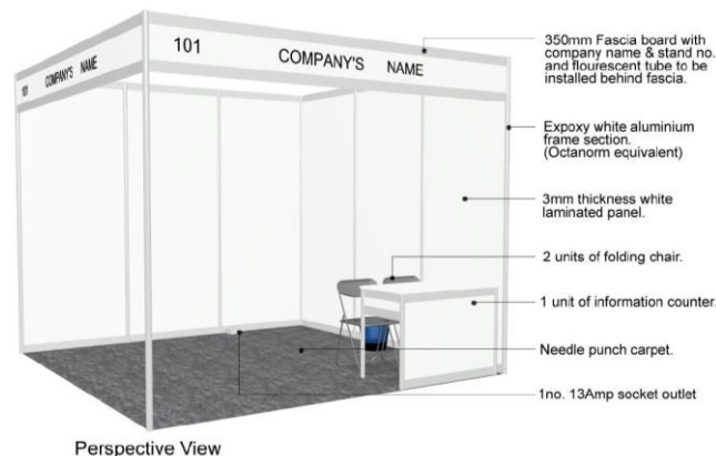
Standard Shell Scheme (3m x 3m)
